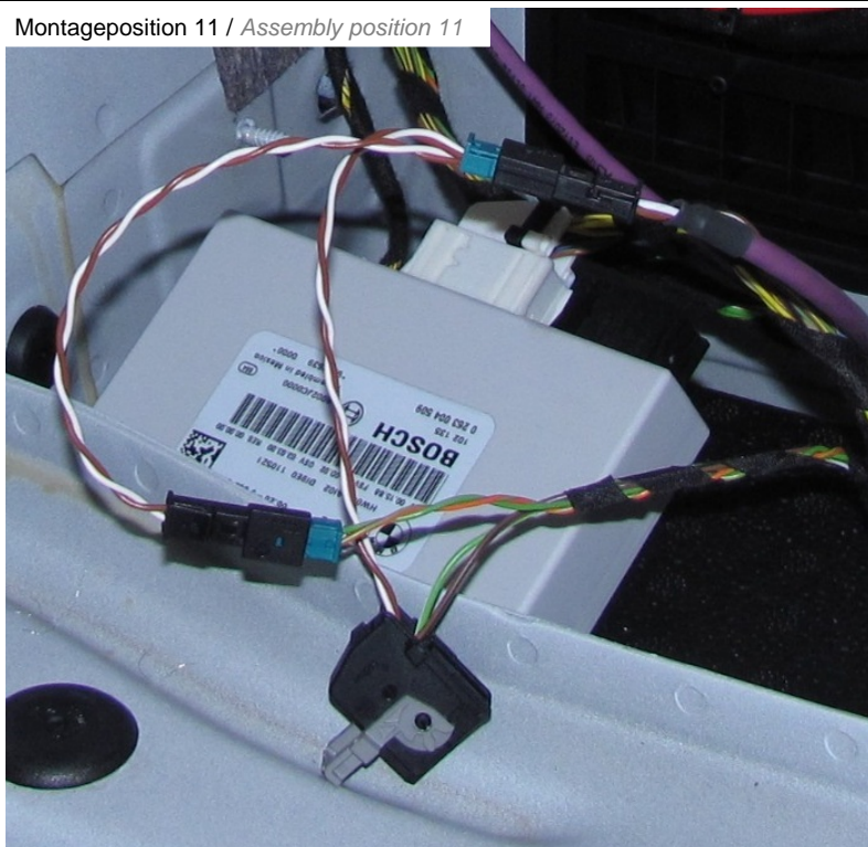
Montageposition 11 / Assembly position 11
