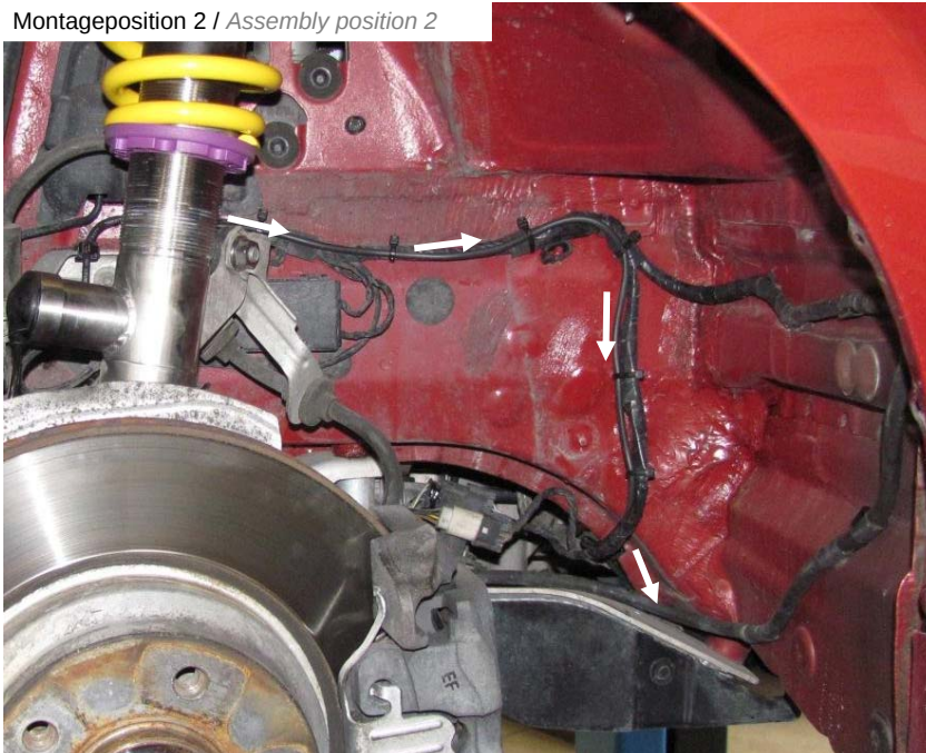
Montageposition 2 / Assembly position 2
