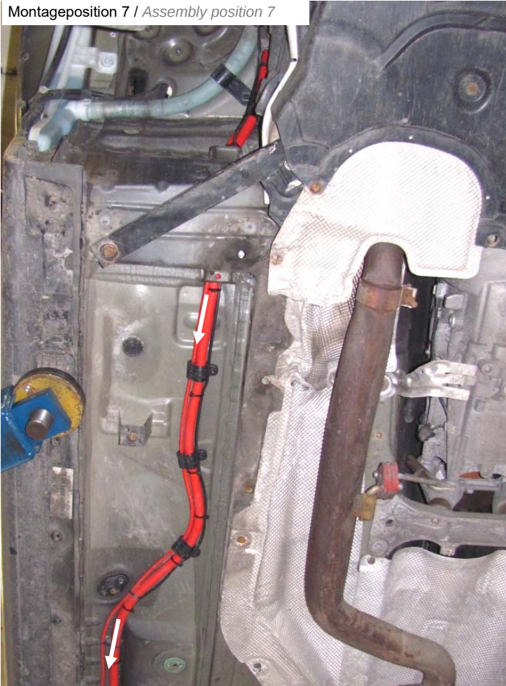
Montageposition 7 / Assembly position 7
