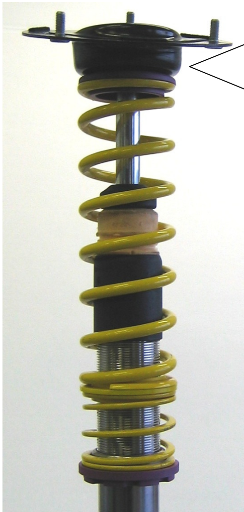
Angeliefertes KW Federbein Supplied KW coilover strut
