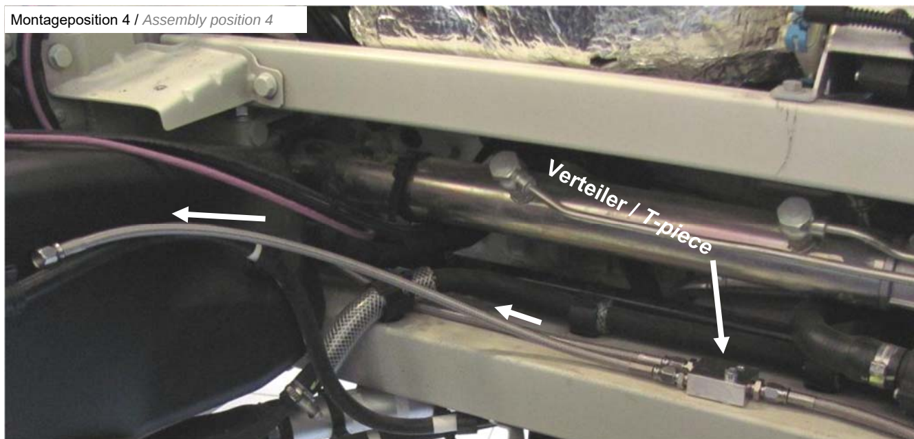
Montageposition 4 / Assembly position 4
