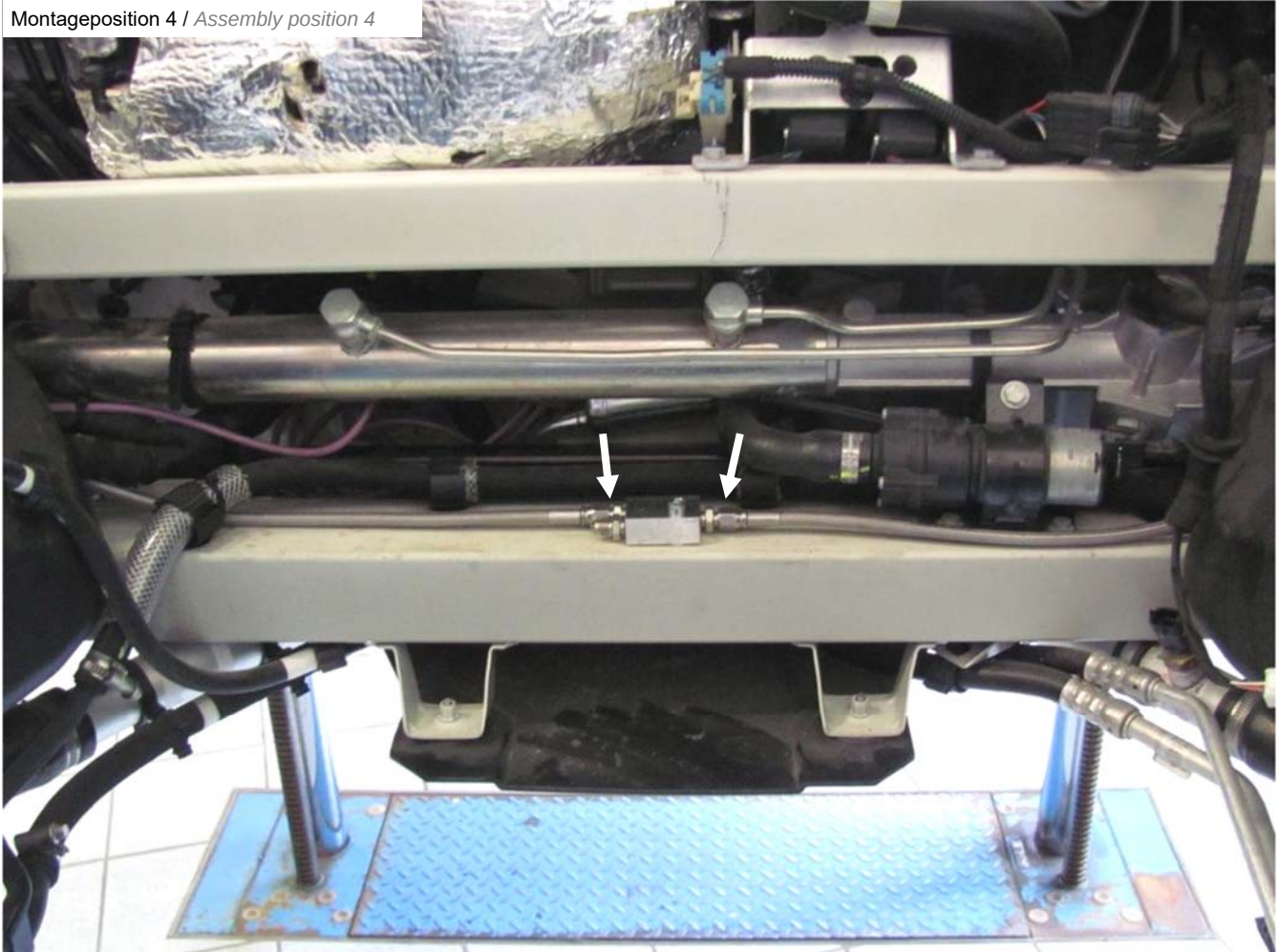
Montageposition 4 / Assembly position 4
