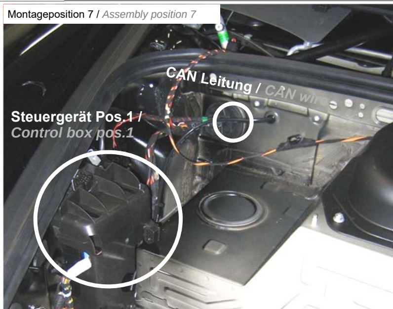
Montageposition 7 / Assembly position 7
