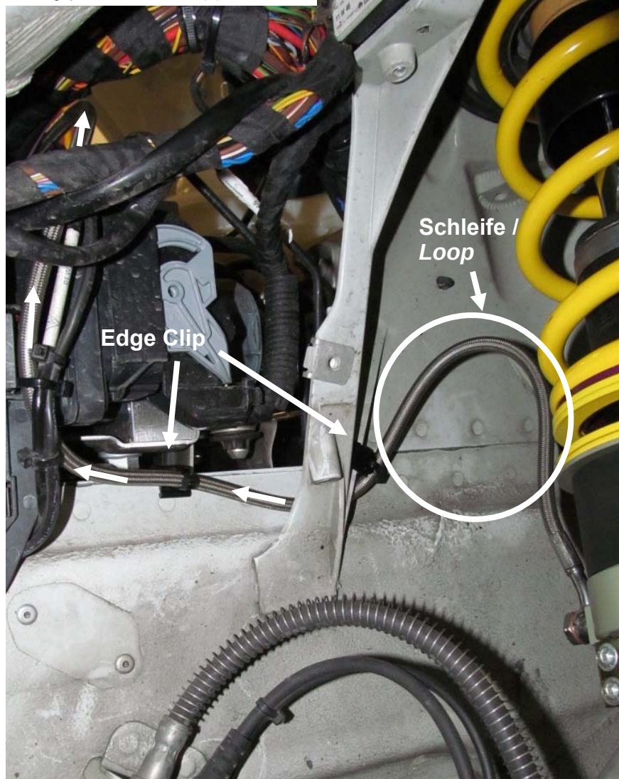
Montageposition 2 / Assembly position 2
