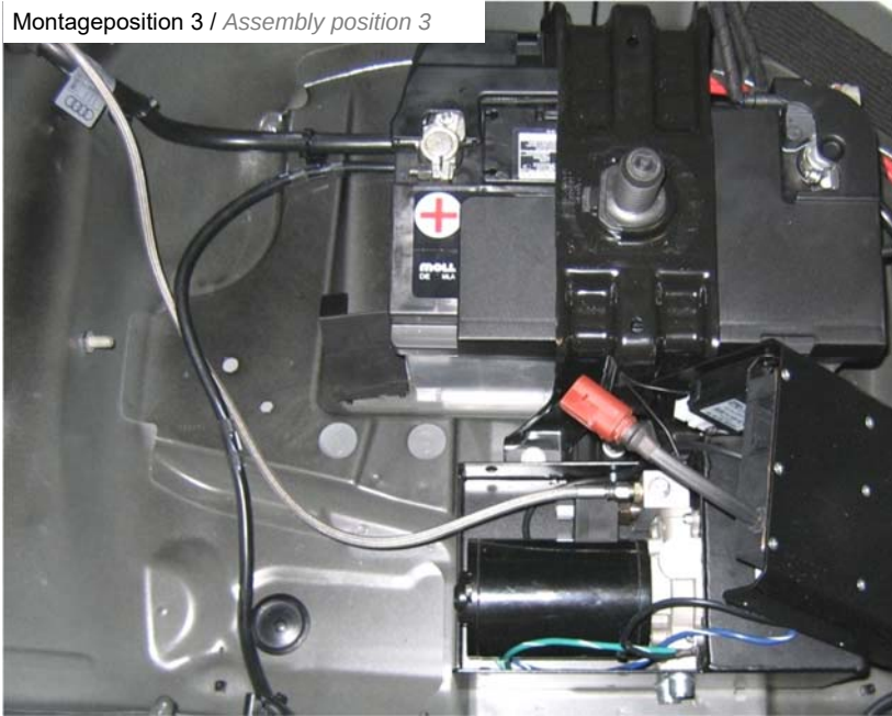
Montageposition 3 / Assembly position 3
