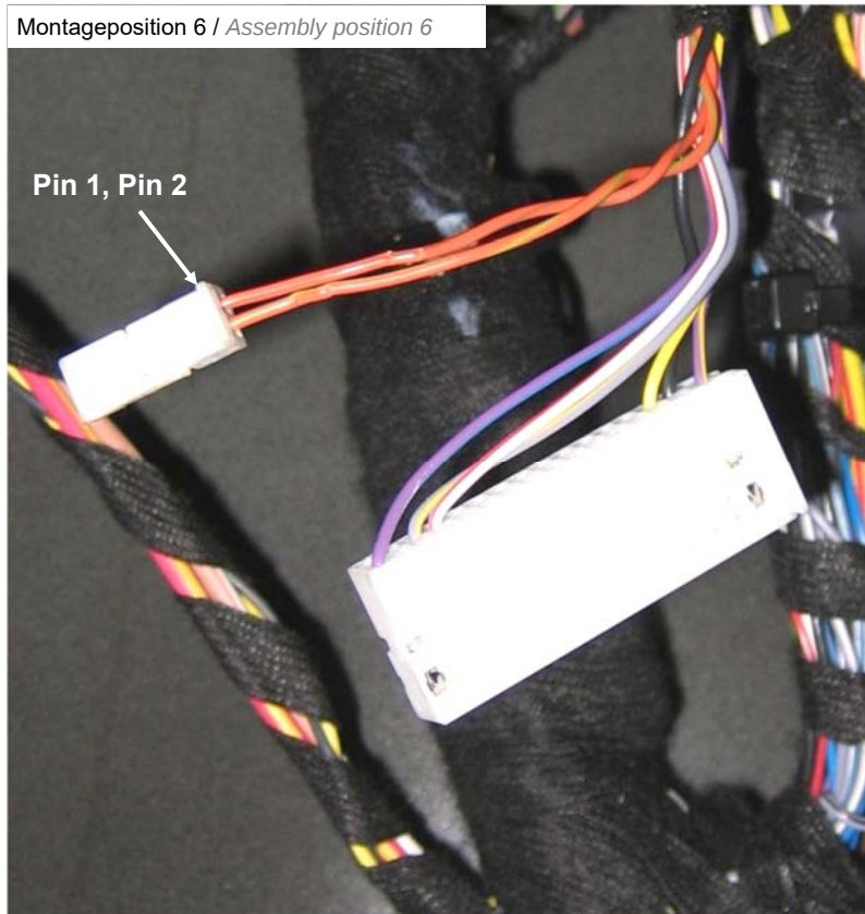
Montageposition 6 / Assembly position 6
